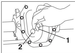
1. Oil level plug 2. Oil level plug hole
