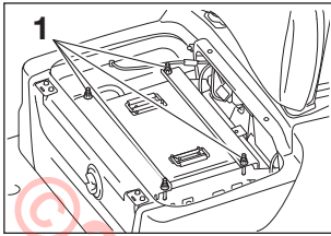
1. Battery hold-down
